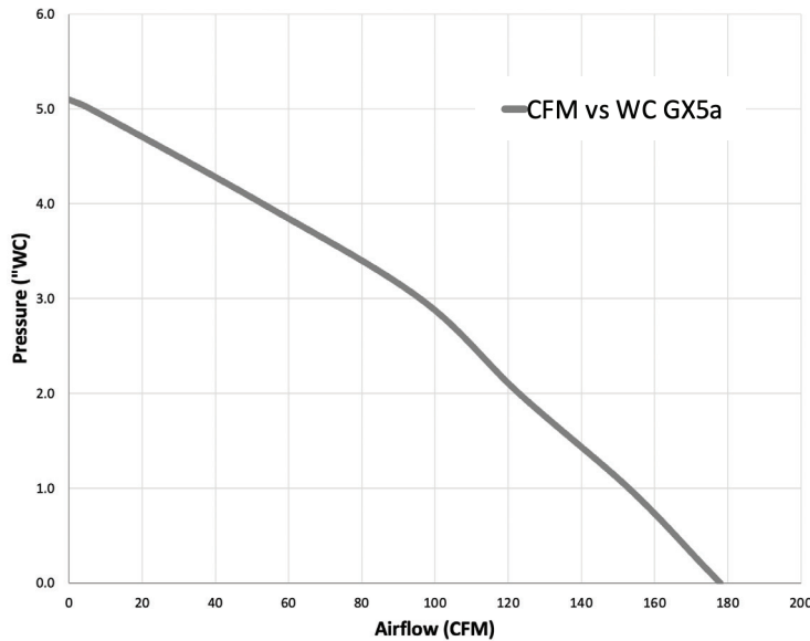
GX5A Performance Curve
