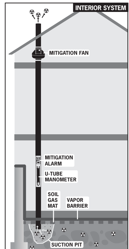
TYPICAL GX5A INDOOR INSTALLATION
