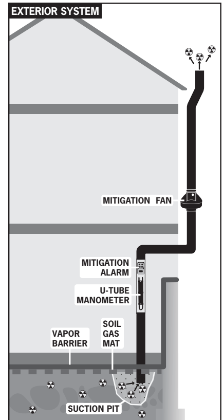
TYPICAL GX5A OUTDOOR INSTALLATION
